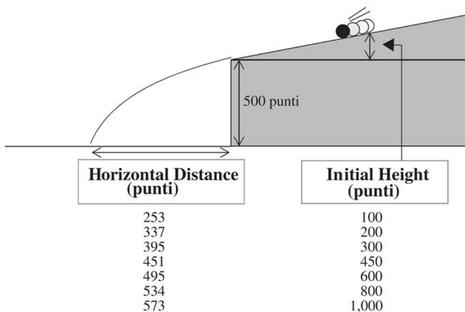
DISPLAY 10.1 Galileo's experimental results
