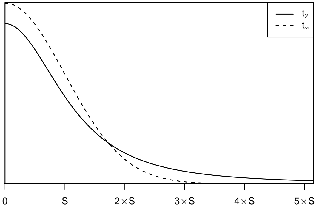
Figure 10.1: The half-t distribution with scale S and 2 degrees of freedom (solid line). The dotted line shows the limit as the degrees of freedom increases to infinity
